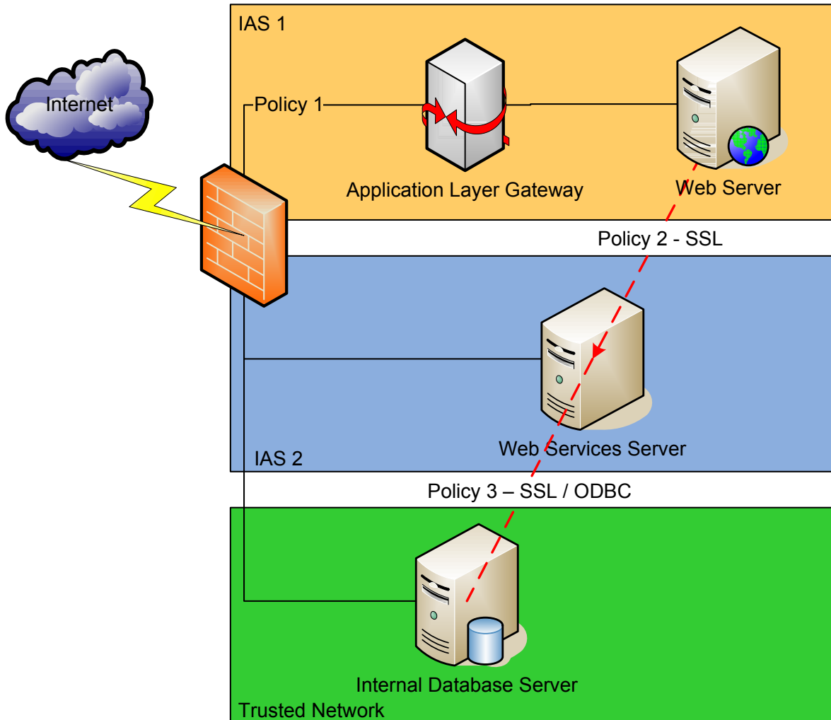
Figure 3: Web Services Design
